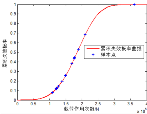
图4 整体搭接壁板结构疲劳寿命分布曲线 Fig. 4 Fatigue life distribution curve of integral lap panel structure
